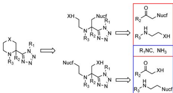
Scheme 1. Retrosynthetic Design of de Novo Assembly of Morpholines and Piperazines by an MCR Approach
